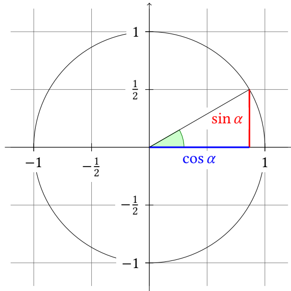
Figure 1.1: A pictorial view of Theorem 1.3.
